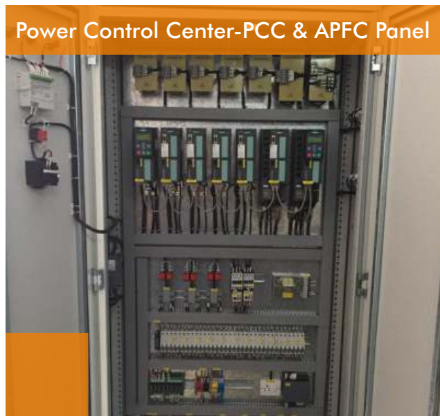
Motor Control Center MCC Panel
